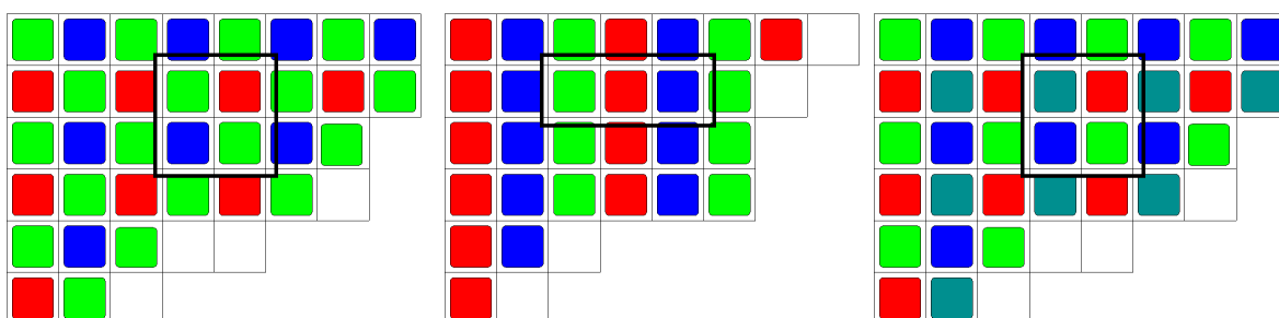
Figure 4 – From left to right : Bayer’s matrix, striped matrix, Sony DSCF628 with 4 colors (one over 2 Green sites is replaced by an Emerald site.) For each matrix, the black box represents the minimal periodic pattern.
